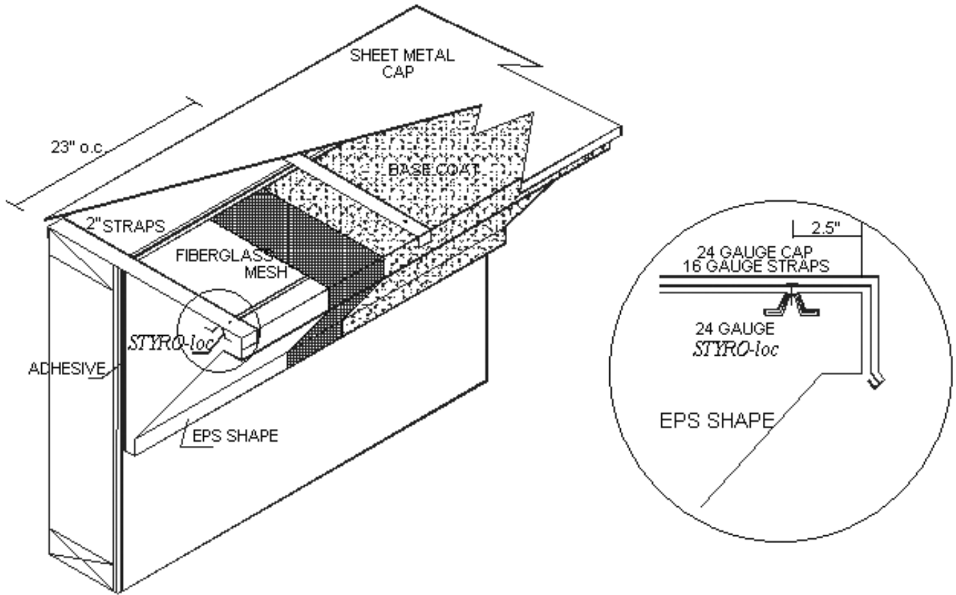
FIGURE 1—STYRO-LOC SYSTEM
