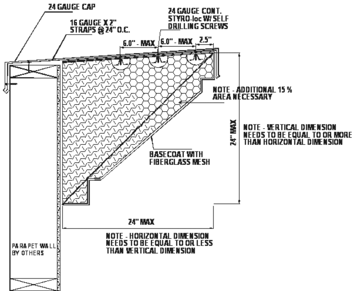
FIGURE 3—SPACING OF STYRO-LOC INSERTS
