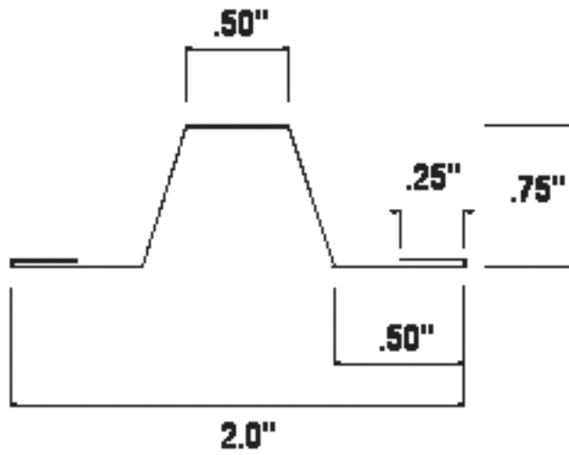
FIGURE 2—STYRO-LOC INSERT
